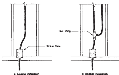
Figure 4.7 Extension of Existing Tubing Run
