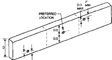
Figure 4.2 Holes in Wood Structures
