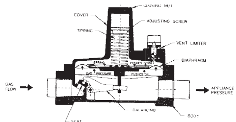
Figure 4.26 Pressure Regulator Diagram
